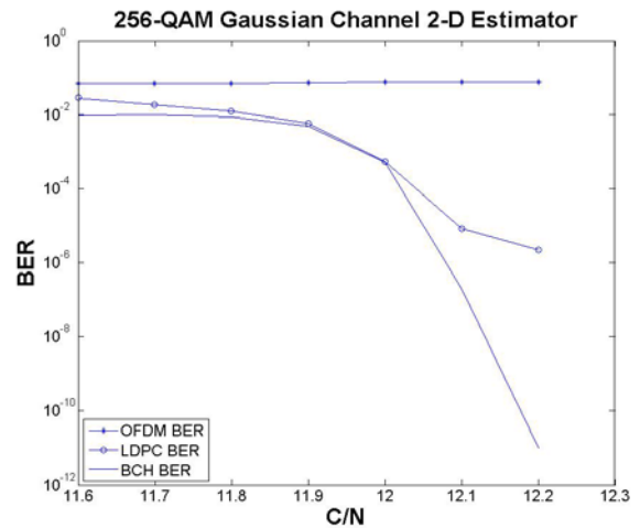
Figure 4: complete simulation of 256QAM performance over Gaussian channel
