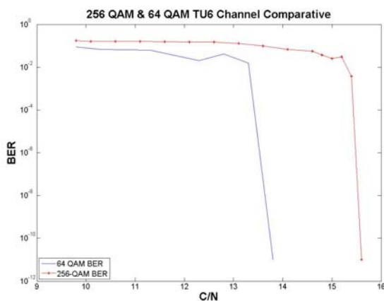
Figure 7: channel comparative for 256QAM
