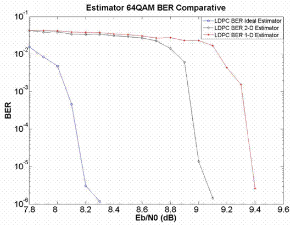
Figure 2: Comparative of channel estimation schemes for F1 channel model
