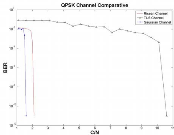
Figure 6: channel comparative for QPS modulation
