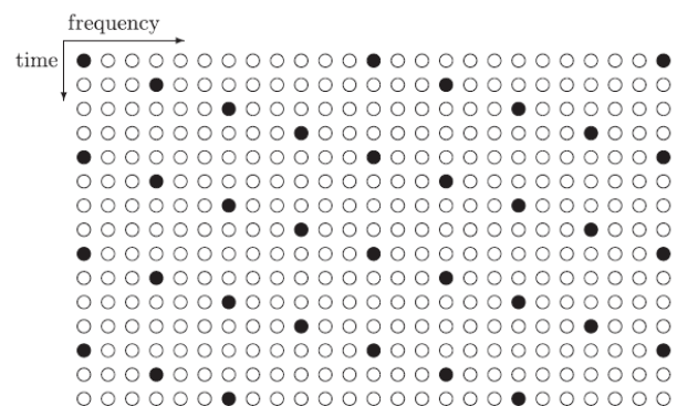
Figure 1 Pilot structure
