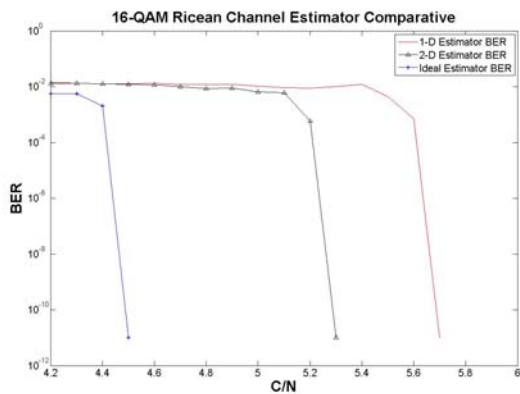
Figure 3: Comparative of channel estimation schemes for F1 channel.
